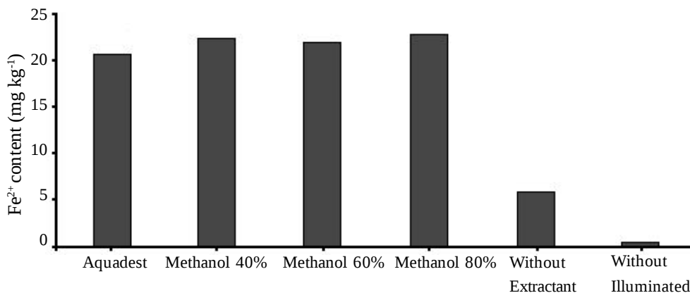
Figure 2. Ferro Concentration on the photoreduction result of clove leaves extract ( Eugenia aromatica ) with aquadest and 40, 60 and 80% methanol solvents in the illuminated box on the photoreduction iron process.
