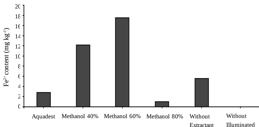
Figure 4. Ferrous concentration of water hyacinth leaves ( Eichhornia crassipes ) with aquadest and 40, 60 and 80% methanol solvents in the illuminated box on the photoreduction iron process.
