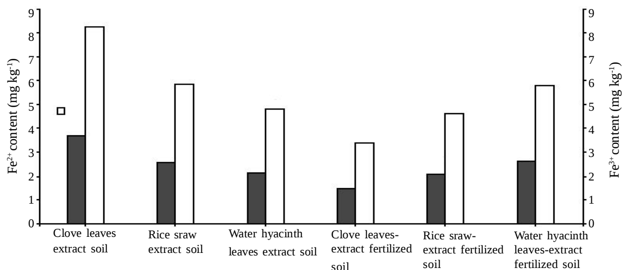
Figure 7. The comparison of Fe 2+ and Fe 3+ concentrations of the soil-extract and soil-fertilizer-extract of clove leaves, rice straw and water hyacinth leaves with 60% methanol in soil media on photoreduction iron process. ■ = Fe 2+ and □ = Fe 3+ concentrations.
