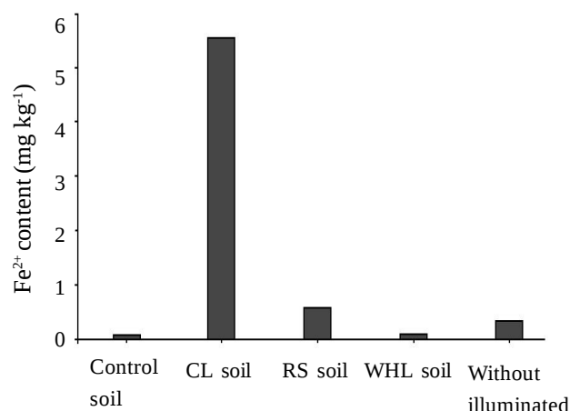
Figure 5. Ferrous concentration of the extract soil of clove leaves (CL) extracted with 80% methanol solvent, rice straw (RS) and water hyacinth leaves (WHL) extracted with 60% methanol solvent in the soil media in the illuminated box of photoreduction iron process.
