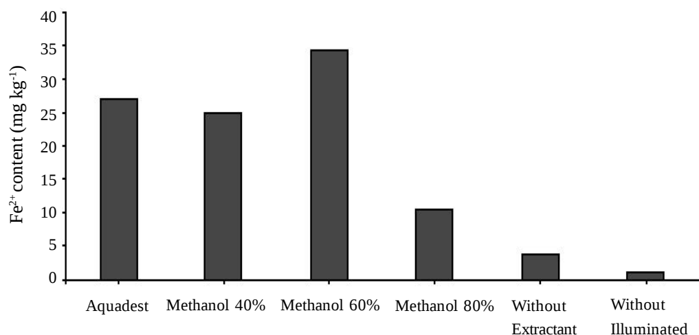
Figure 3. Ferrous concentration of Rice Straw with aquadest and 40, 60 and 80% methanol solvents in the illuminated box on the photoreduction iron process.
