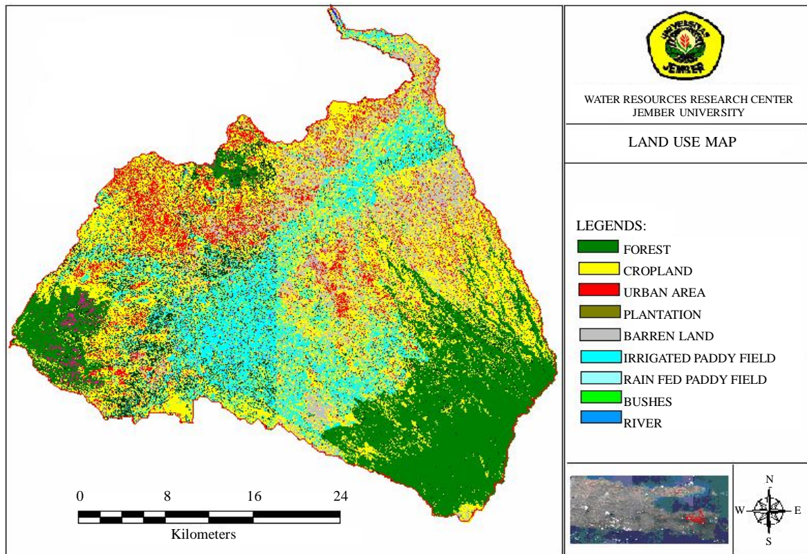
Figure 8. Land Use Map in Sampean Watershed obtained from supervised classification.
