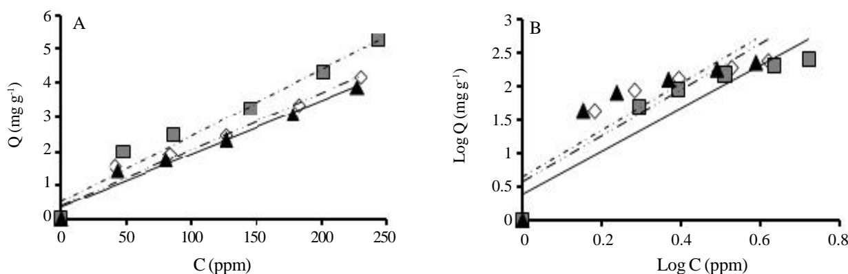
Figure 4. The equation of Langmuir isotherm (A) and Freundlich (B) heavy metals Pb 2+ , Cu 2+ and Cd 2+ by ZSM-5 zeolite. ◇ : Cu, ■ : Cd, ▲ : Pb.
