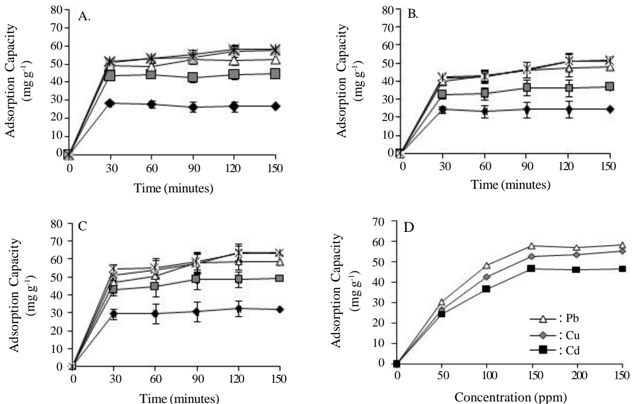
Figure 3. Metal adsorption by ZSM-5 at various concentration and contact time (A) Cu 2+ ; (B) Cd 2+ ; (C) Pb 2+ and (D) fitting adsorption capacity by ZSM-5 to metals Pb 2+ , Cu 2+ and Cd 2+ . \blacklozenge : 50 ppm, \blacksquare : 100 ppm, \blacktriangle : 150 ppm, \blackstar : 200 ppm, \blacktimes : 250 ppm.
