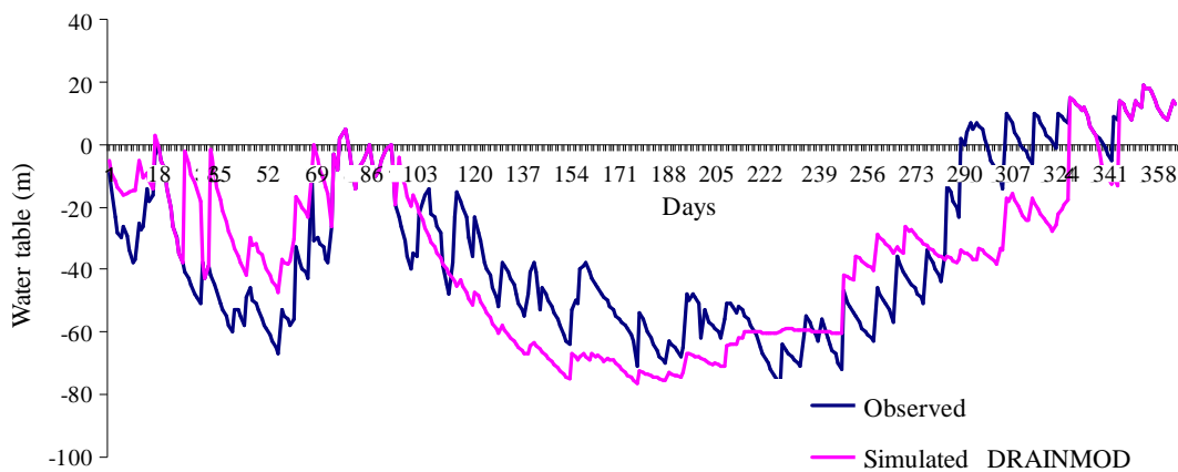
Figure 6. Water table dynamics pattern from computer simulation of DRAINMOD and field measurements.
