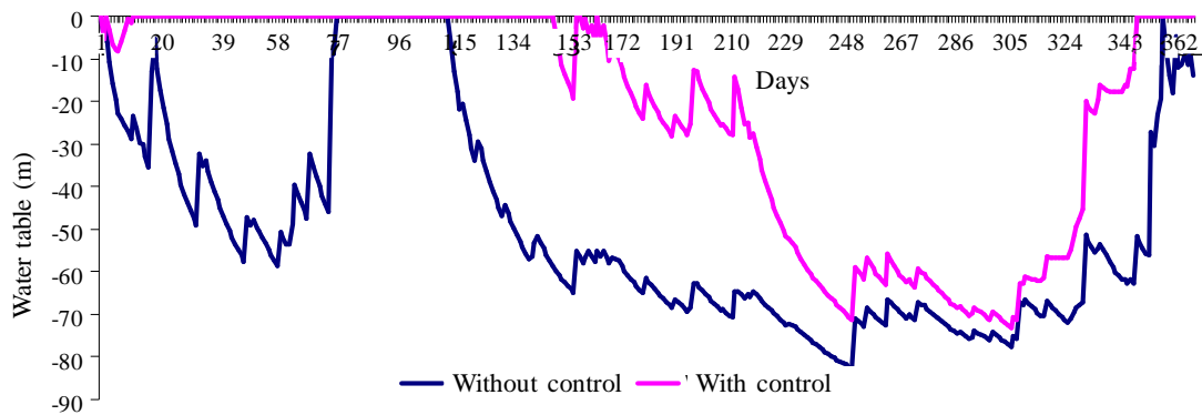
Figure 8. Results of DRAINMOD simulation in term of water gate effect on water table control for corn crop.
