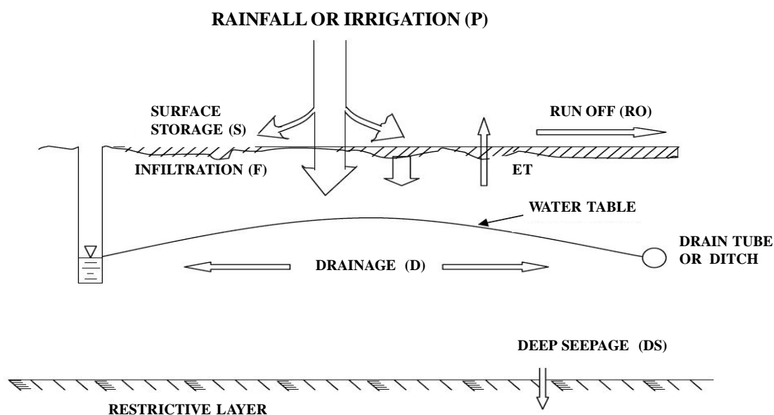
Figure 2. Components of water balance in DRAINMOD model (Skaggs 1991).
