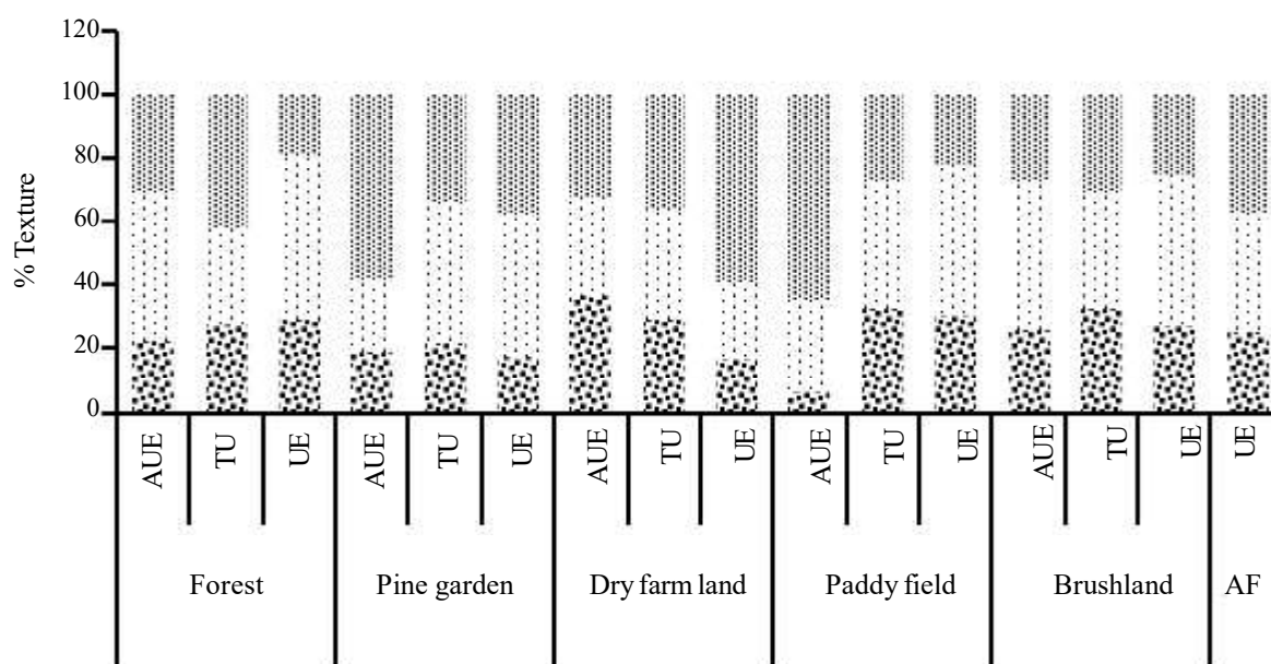
Figure 3. Soil texture at 30-60 cm depth. Description: AUE: Anthropic Udic Eutrandepts; TU: Typic Ustrolepts; UE: Udic Eutrandepts. ■ : % sand, ■ : %silt, ■ : % clay.
