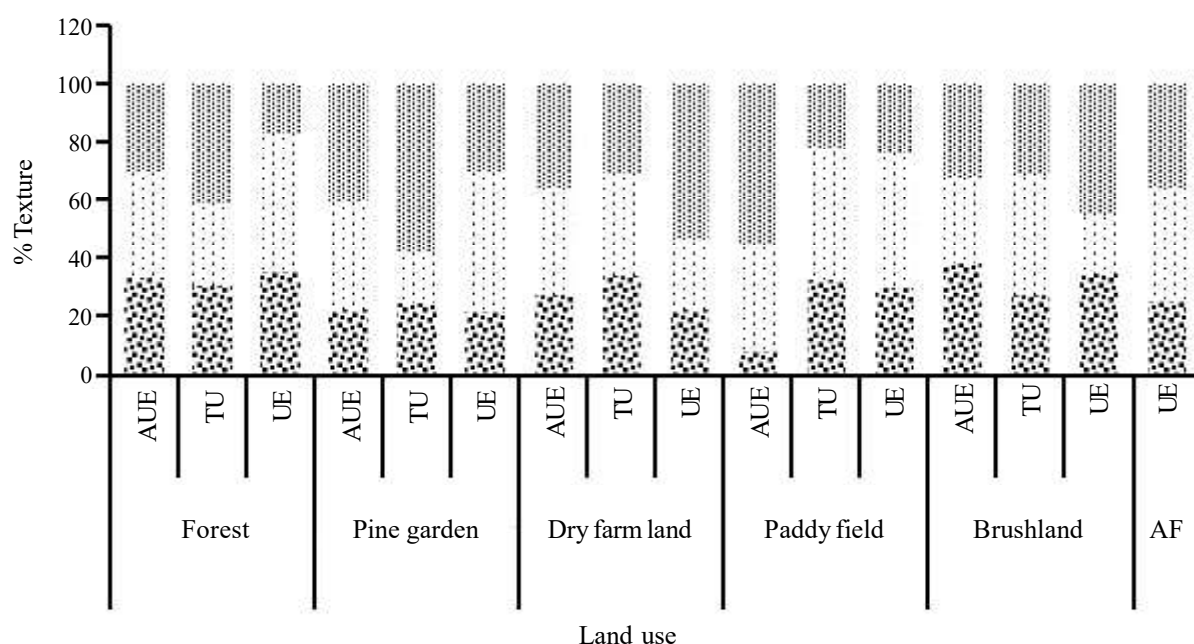
Figure 2. Soil texture at 0-30 cm depth. Description: AUE: Anthropropic Udic Eutrandedpts; TU: Typic Ustropepts; UE: Udic Eutrandedpts. ■ : % sand, ■ : %silt, ■ .
