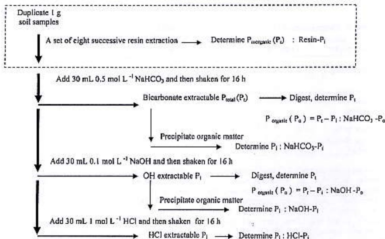
Figure 1. Flow chart of the P fractionation into various inorganic- and organic-P fractions.
