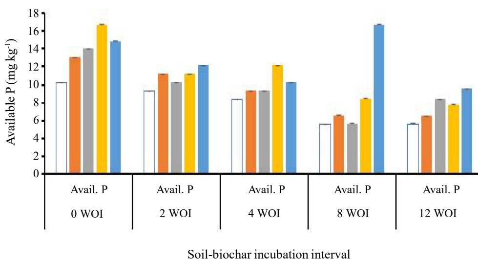
Figure 3. Effects of rice-husk biochar on available P content of the soil under the different soil-biochar incubation intervals. Error bars represent LSD at a 5% probability level ( LSD_{0.05} ). □ : 0 Mg ha -1 , ■ : 7.5 Mg ha -1 , ■ : 15 Mg ha -1 , ■ : 30 Mg ha -1 , ■ : 60 Mg ha -1 .
