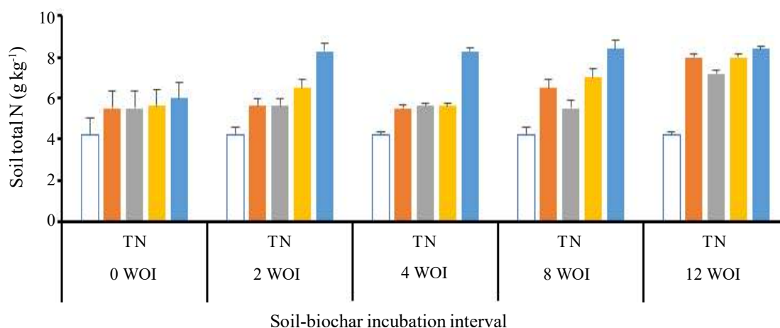
Figure 2. Effects of rice-husk biochar on soil total N under the different soil-biochar incubation intervals. Error bars represent LSD at a 5% probability level ( LSD_{0.05} ). □ : 0 Mg ha -1 , ■ : 7.5 Mg ha -1 , ■ : 15 Mg ha -1 , ■ : 30 Mg ha -1 , ■ : 60 Mg ha -1 .
